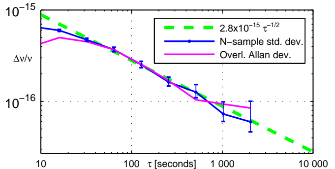
FIG. 2: Clock stability. Fractional frequency uncertainty vs. averaging period ( \tau ) for a comparison between the two \text{Al}^+ clocks (10700 s duration). Overlapping Allan deviation and N-sample standard deviation are shown [22]. For each comparison measurement the coefficient of the \tau^{-1/2} asymptote is estimated and used to derive the measurement's statistical uncertainty. The 2.8 \times 10^{-15} \tau^{-1/2} asymptote is reached for averaging periods that are longer than the servo time constant of 10 s.
