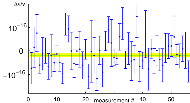
FIG. 3: Measurements of the fractional frequency difference between the two \text{Al}^+ clocks (blue points). Error bars represent the statistical uncertainty (see Fig. 2). The horizontal line shows the weighted mean of -1.8 \times 10^{-17} with an overall statistical uncertainty of \pm 7.0 \times 10^{-18} (shaded band).
