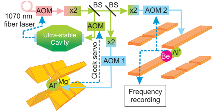
FIG. 1: Setup for comparing the frequencies of the two \text{Al}^+ clocks. The 4 th harmonic of a fiber laser is locked to the \text{Al}^+ ^1\text{S}_0 \leftrightarrow ^3\text{P}_0 clock transition in the Al-Mg apparatus with a fixed offset frequency (applied to AOM1). Another laser beam derived from the same laser probes the clock transition in the Al-Be apparatus, where the laser frequency is locked to the clock transition in a separate digital feedback loop that controls AOM2. The record of frequencies applied to AOM2 represents the difference in clock frequencies. BS: beam splitter; AOM: acousto-optic modulator; x2: frequency doubler.
